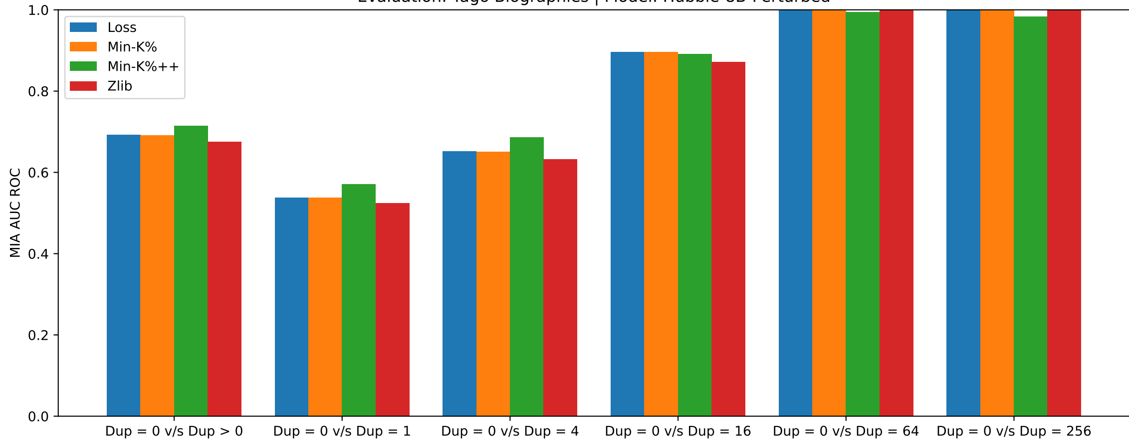
Evaluation: Yago Biographies | Model: Hubble-8B-Perturbed
